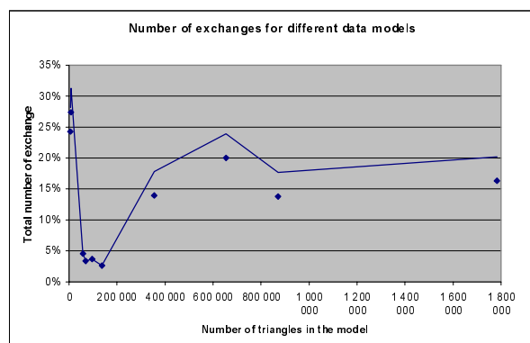
Edges exchanges of the triangular mesh
